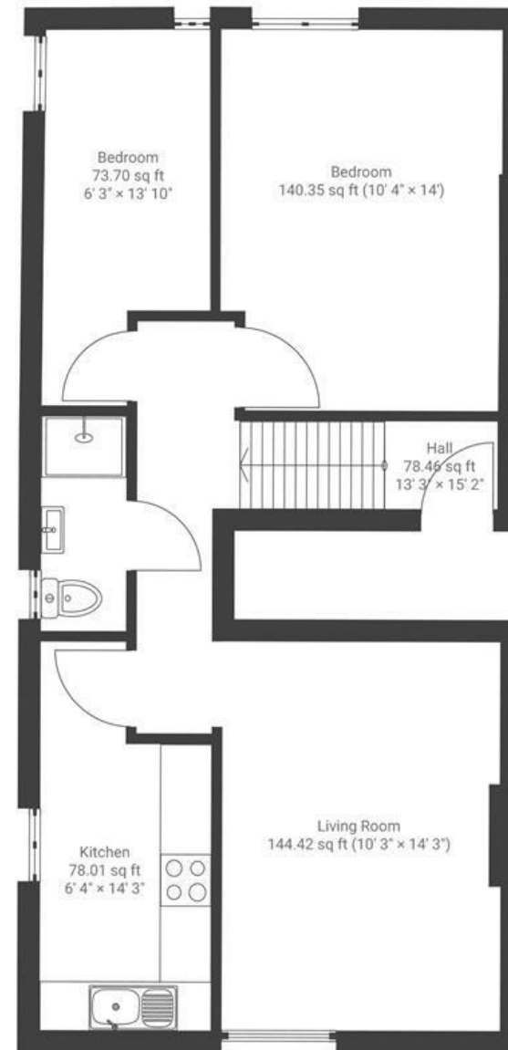
THIRD FLOOR
